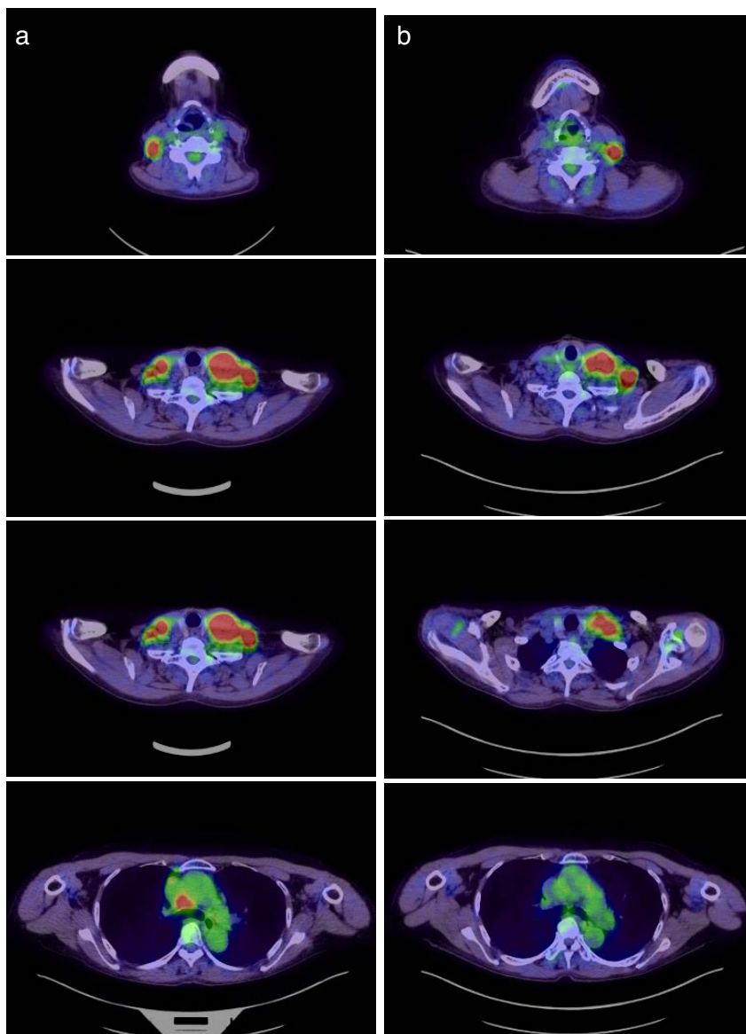
図3 PET-CT
